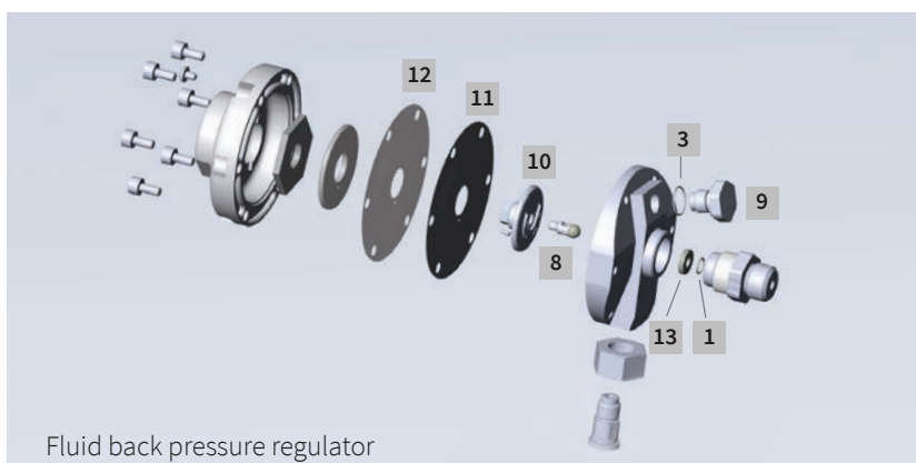
Fluid pressure regulator
